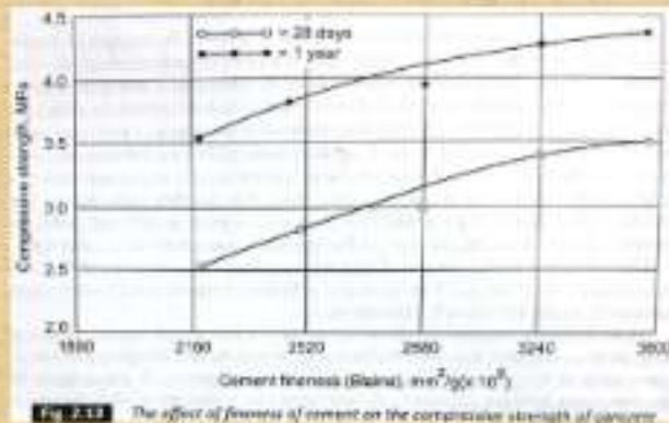
FIGURE 2.13 The effect of fineness of cement on the compressive strength of concrete
